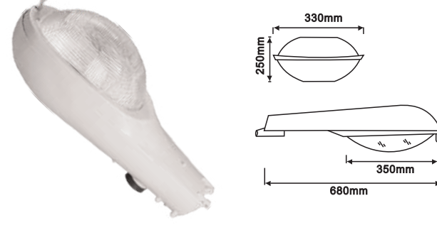
PHFR-250B E40 150W/250W/400W
